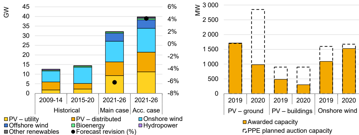
Figure 1.27 France renewable capacity additions, 2009-2026 (left), and auction results, 2019-2020 (right)
